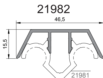
angular cover pr
