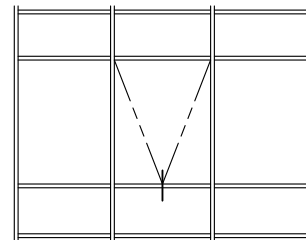
horizontal thermal break opening with glazing bead
