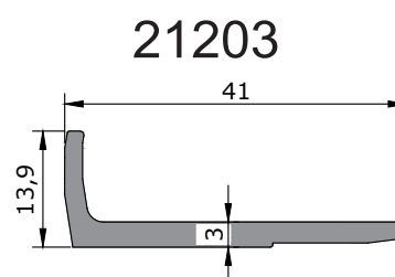
glass support profile
