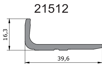
glass support profile
