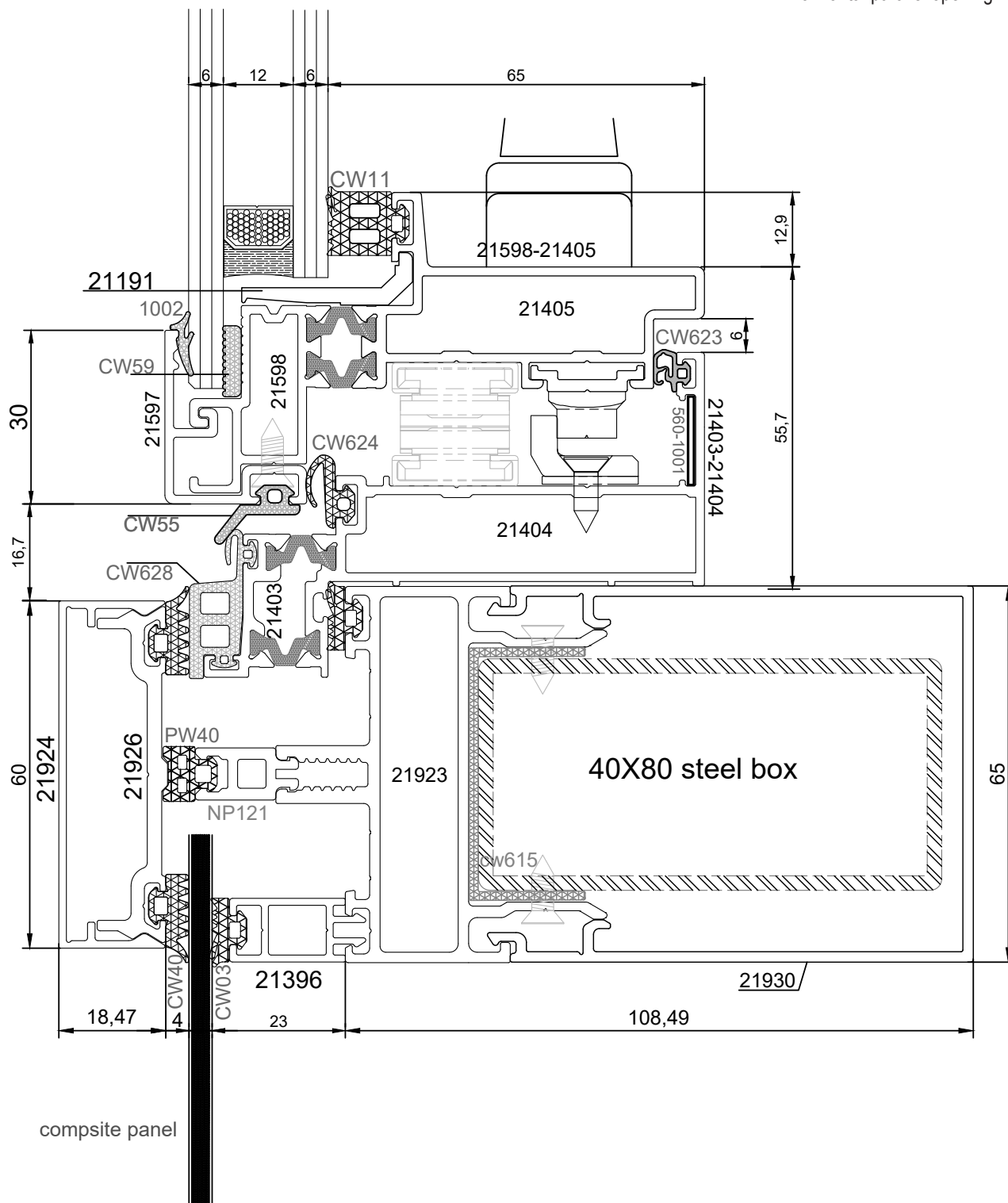
horizontal parallel opening
