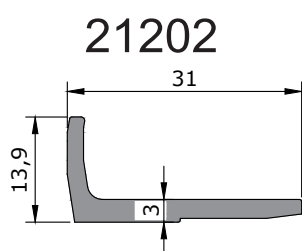
glass support for 60mm transom
