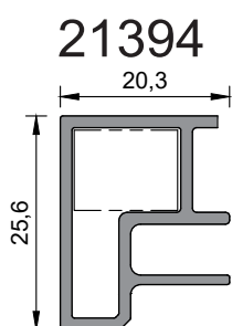
single glass bonding pr
