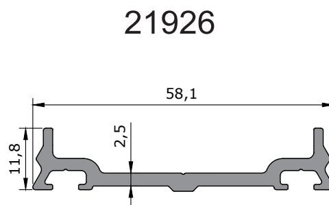
pressure plate profile
