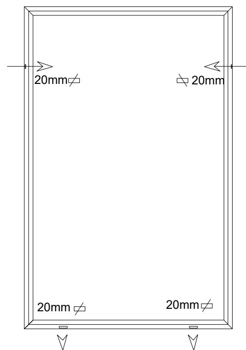
drainage and ventilation schema
