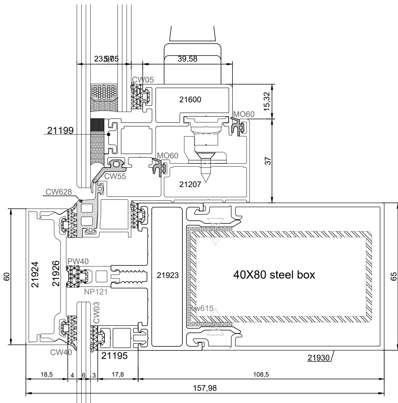
horizontal normal opening
