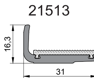
glass support profile
