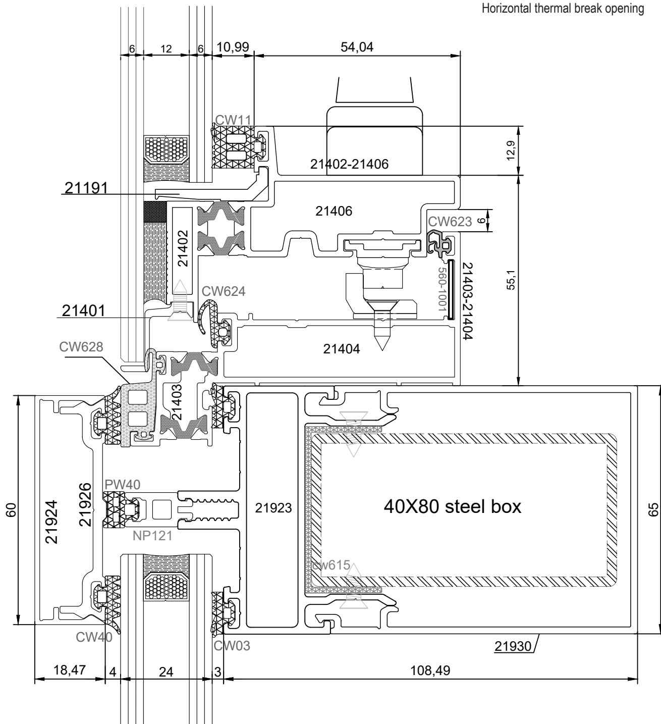
Horizontal thermal break opening
