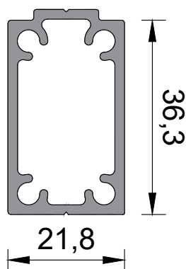
adapter profile
