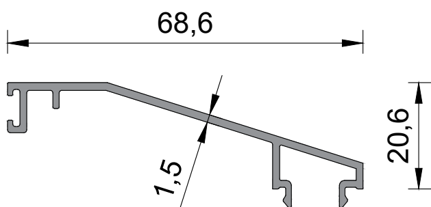
cover profile
