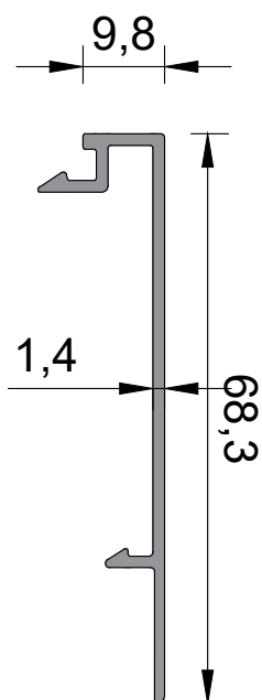
interlock profile
