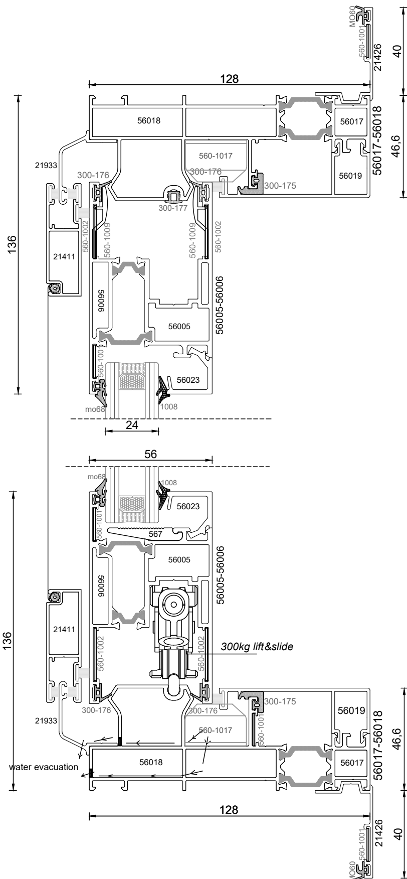
lift & slide-300 kg
