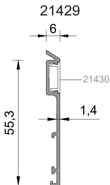
adapter profile
