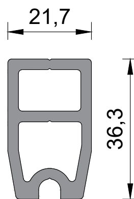
small sash fixing profile
