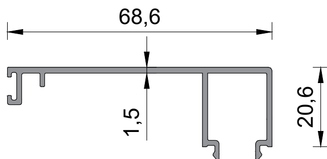
adapter profile
